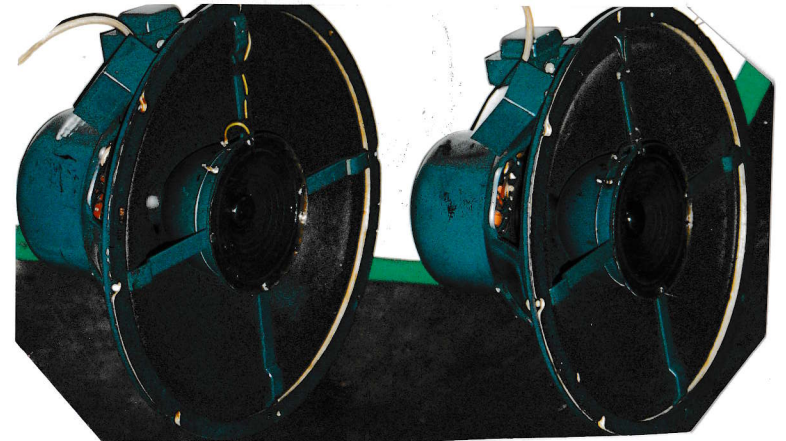
JHP-52 System Corner D-Oak Jensen AA 38cm 同軸 2way JHP-52 220049 - 220048
